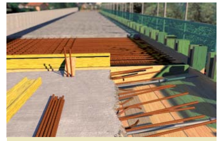
Rebar connections
